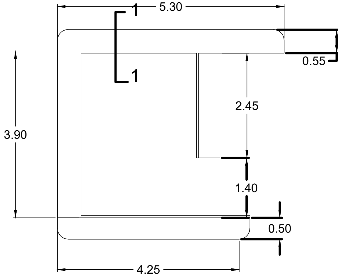
PLAN OF LAMINATED COMPUTER TABLE IN IT LAB.
