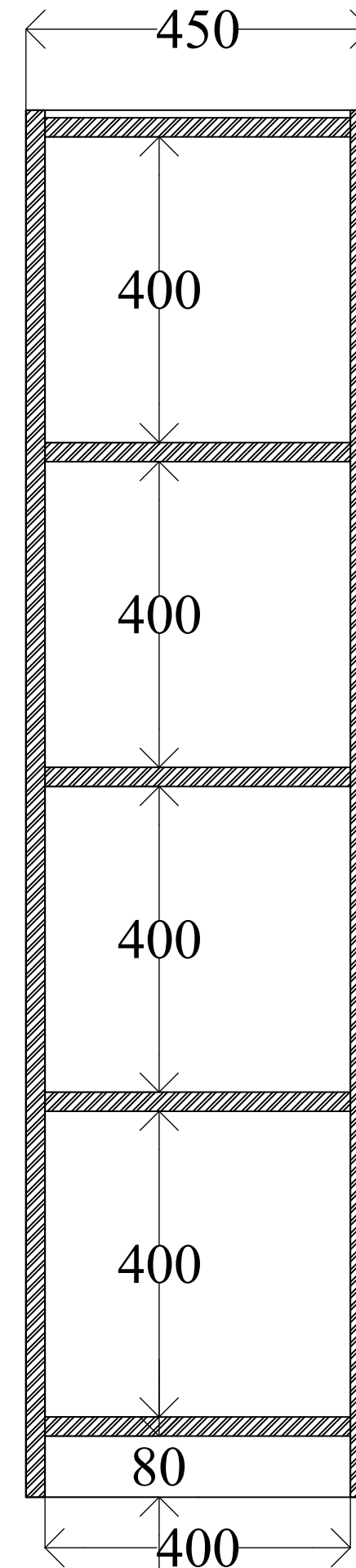
CROSS SECTION
