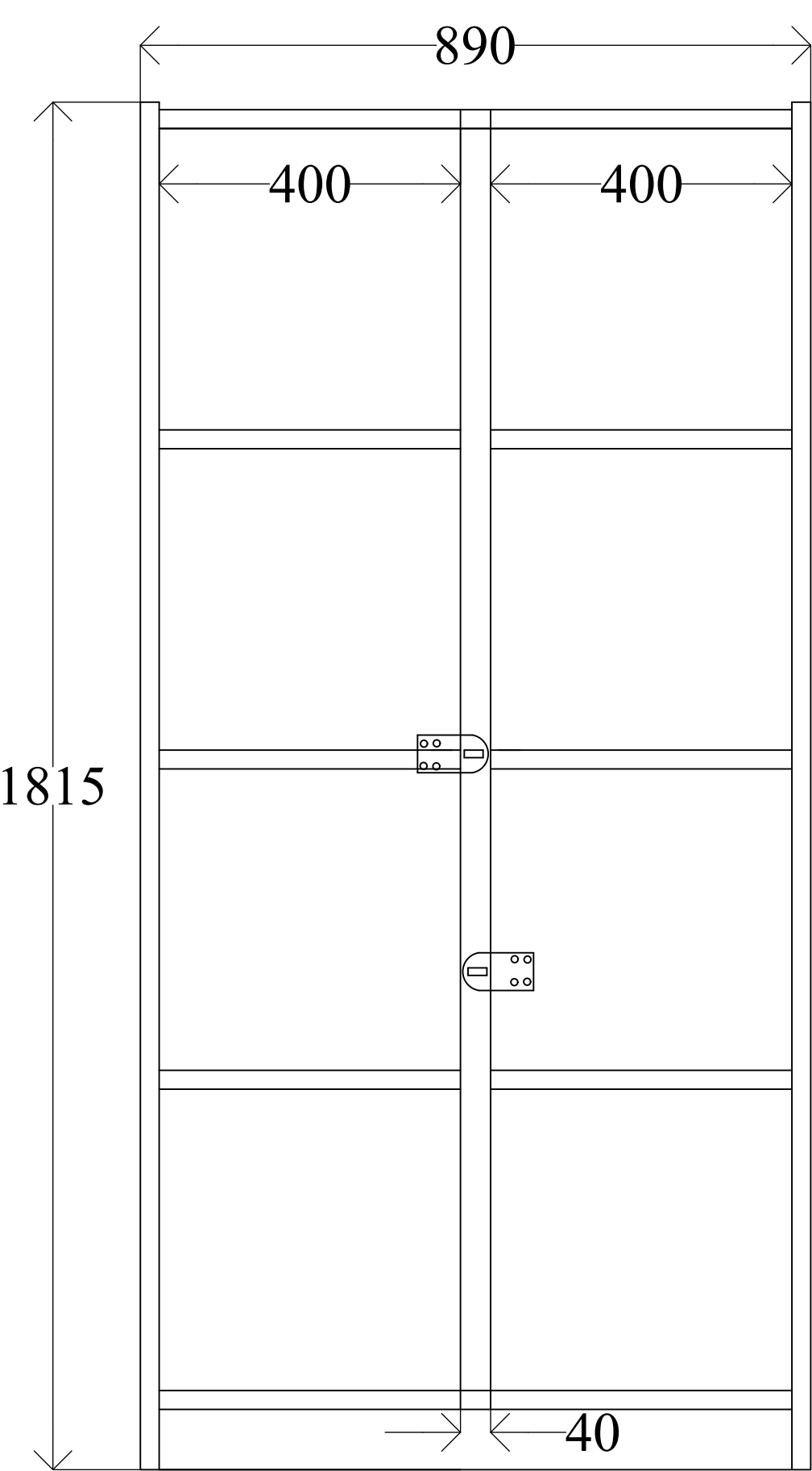
CUPBOARD PLAN
