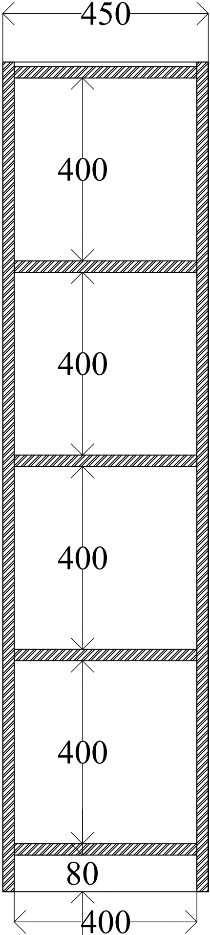
CROSS SECTION
